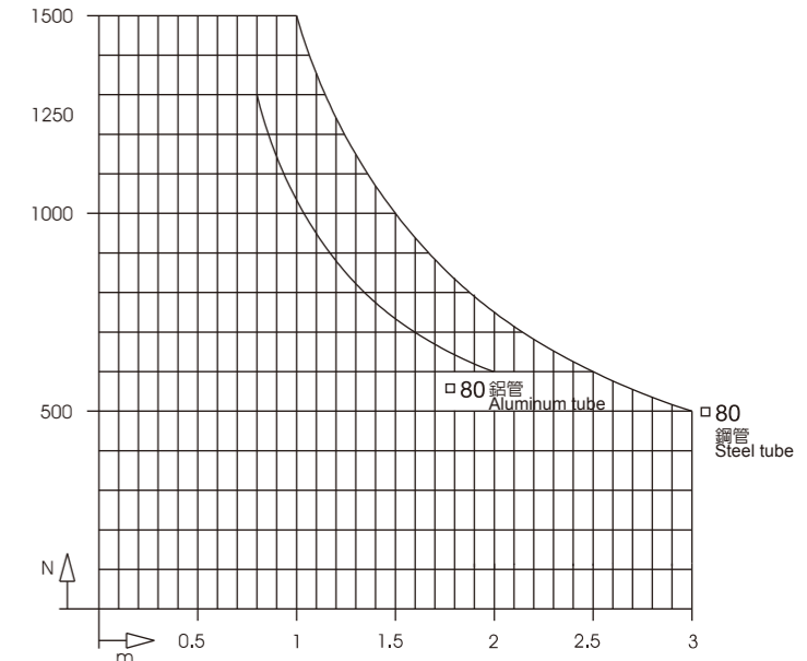
80系列重型懸臂承重力圖 Load - bearing chart of 80 series heavy support arm
