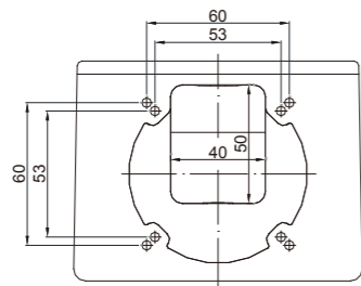
DA901接線盒安裝尺寸 Installation size of DA901 terminal box
