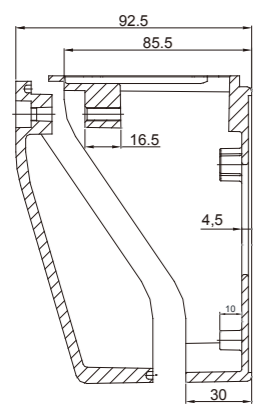
DA901接線盒安裝尺寸 Installation size of DA901 terminal box
