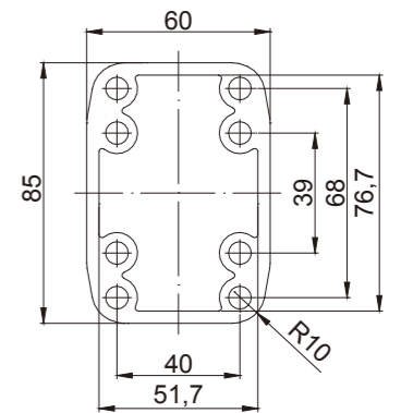
6085鋁管規格表(配6085懸臂): Size table of 6085 aluminum tubes ( for 6085 support arms)
