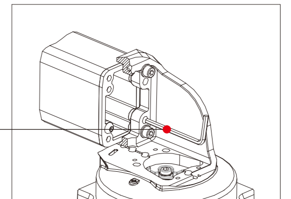
調節連接管水平度 Adjusting levelness of the connecting tube
